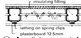
② Acoustic improvement of floor
